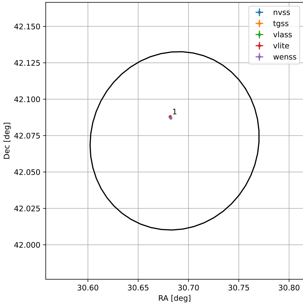
4FGL J0202.7+4204
