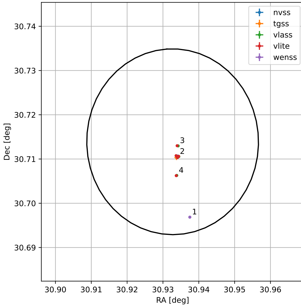
4FGL J0203.7+3042
