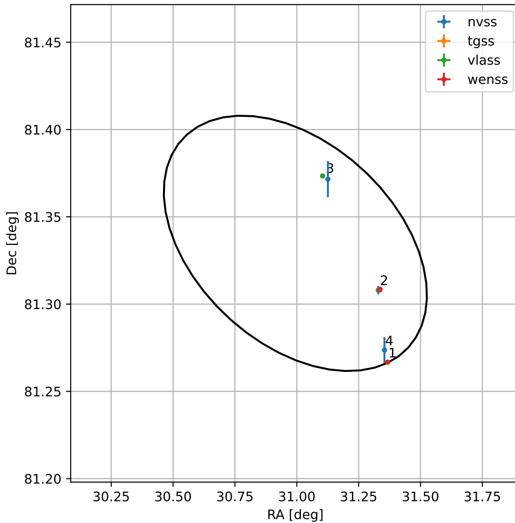
4FGL J0203.9+8120
