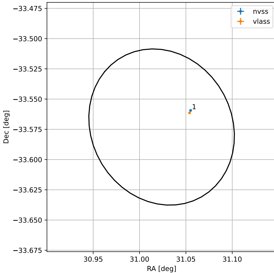
4FGL J0204.0-3334
