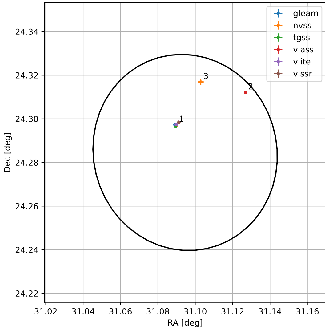
4FGL J0204.3+2417
