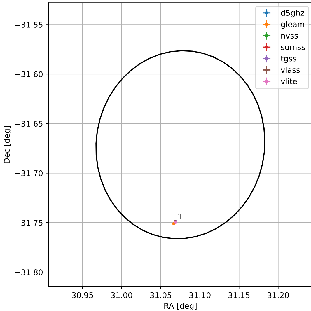
4FGL J0204.3-3140
