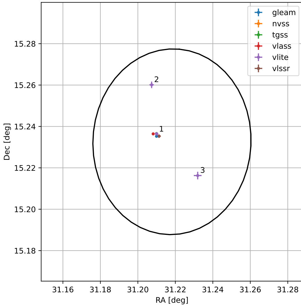
4FGL J0204.8+1513
