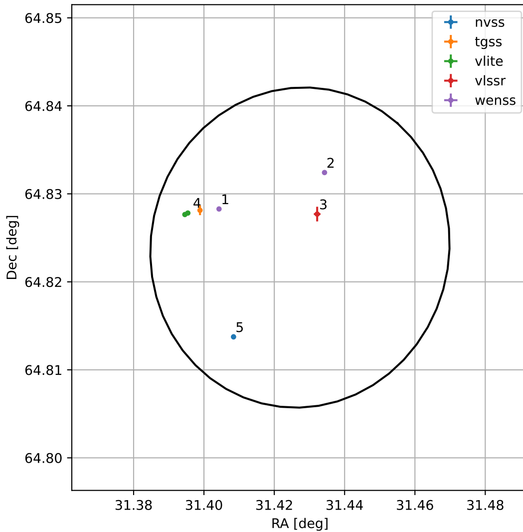
4FGL J0205.7+6449
