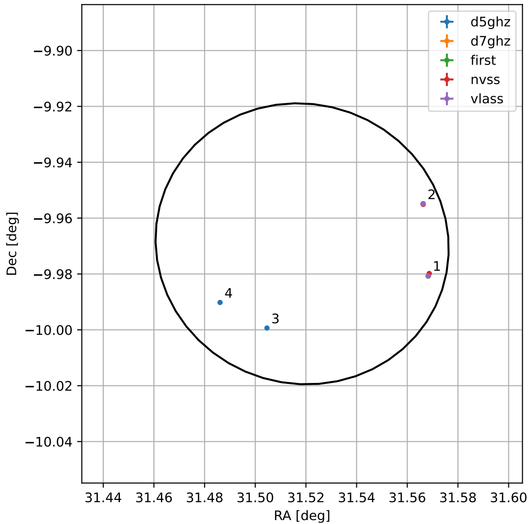
4FGL J0206.0-0958
