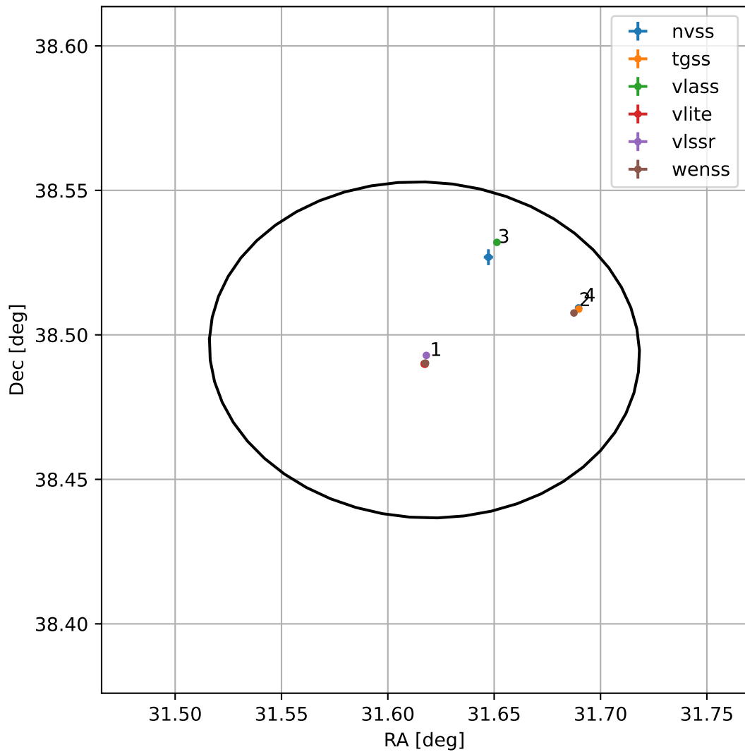
4FGL J0206.4+3829
