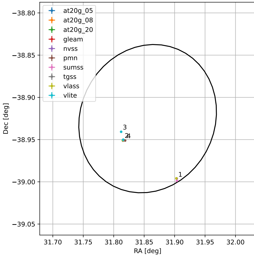
4FGL J0207.4-3855
