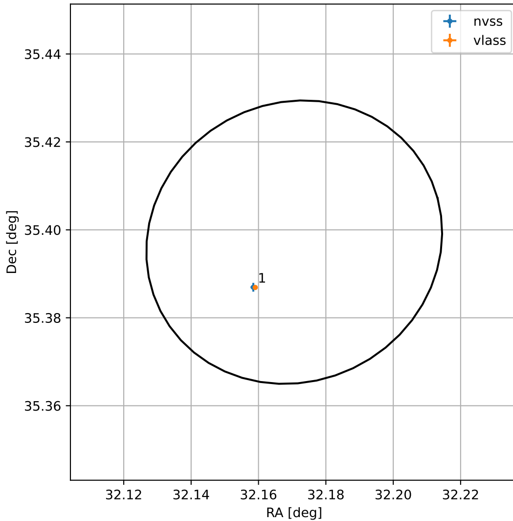
4FGL J0208.6+3523
