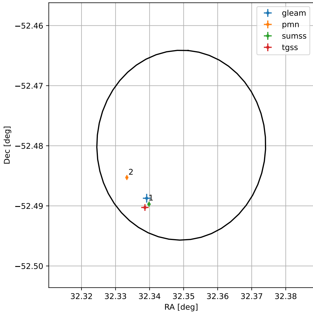
4FGL J0209.3-5228
