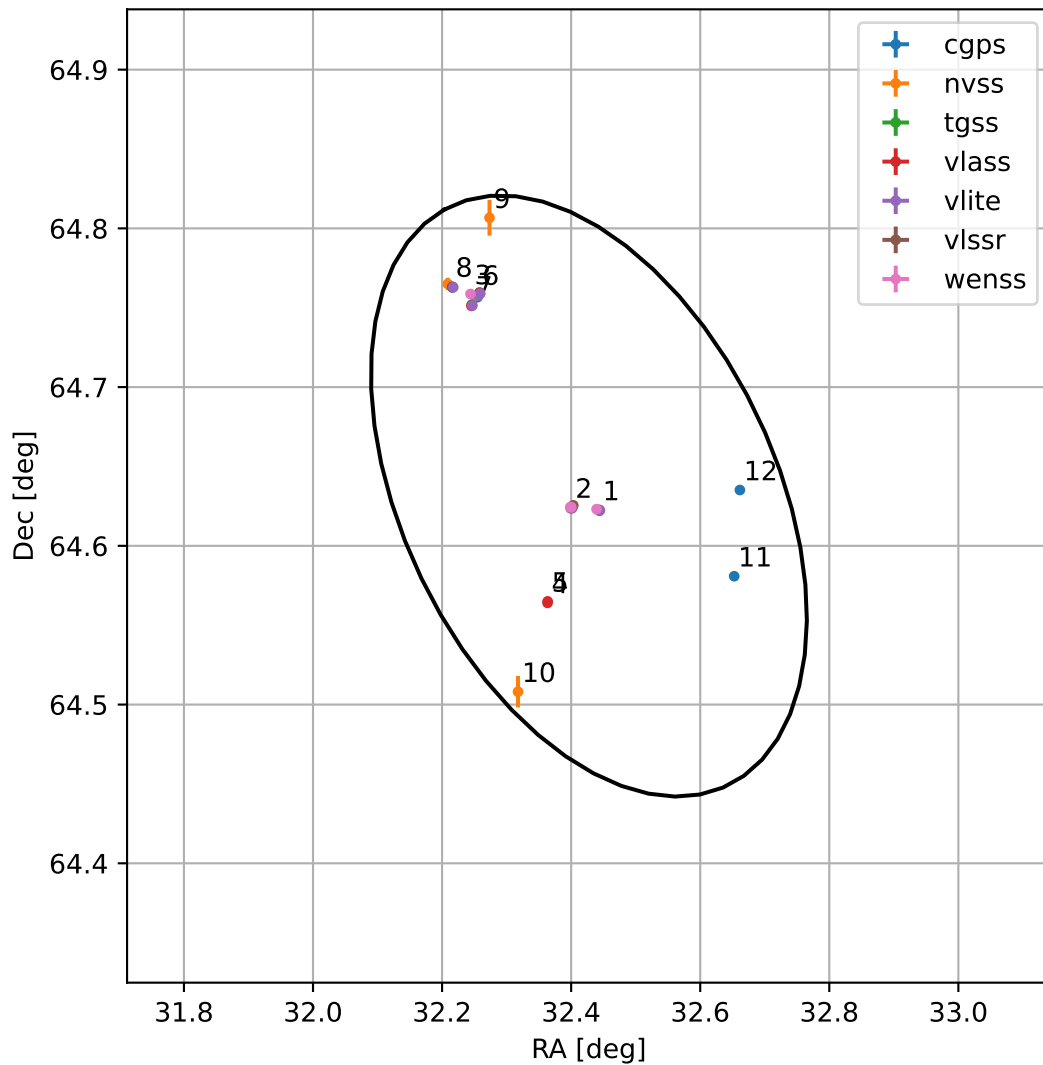
4FGL J0209.7+6437
