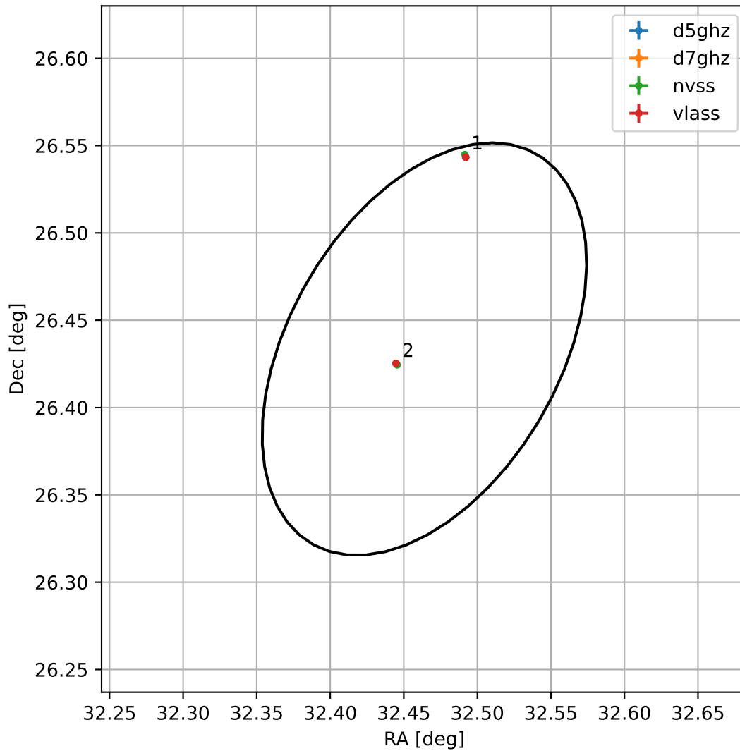
4FGL J0209.8+2626
