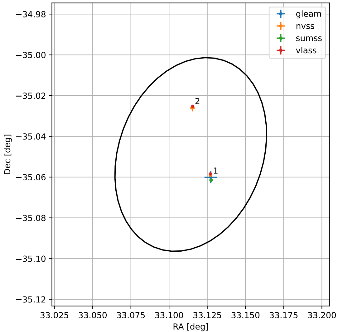
4FGL J0212.4-3502
