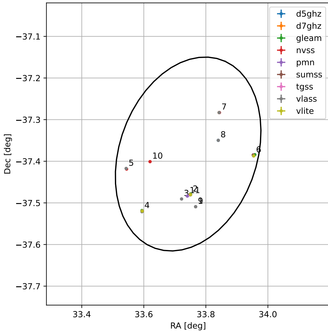
4FGL J0214.9-3722
