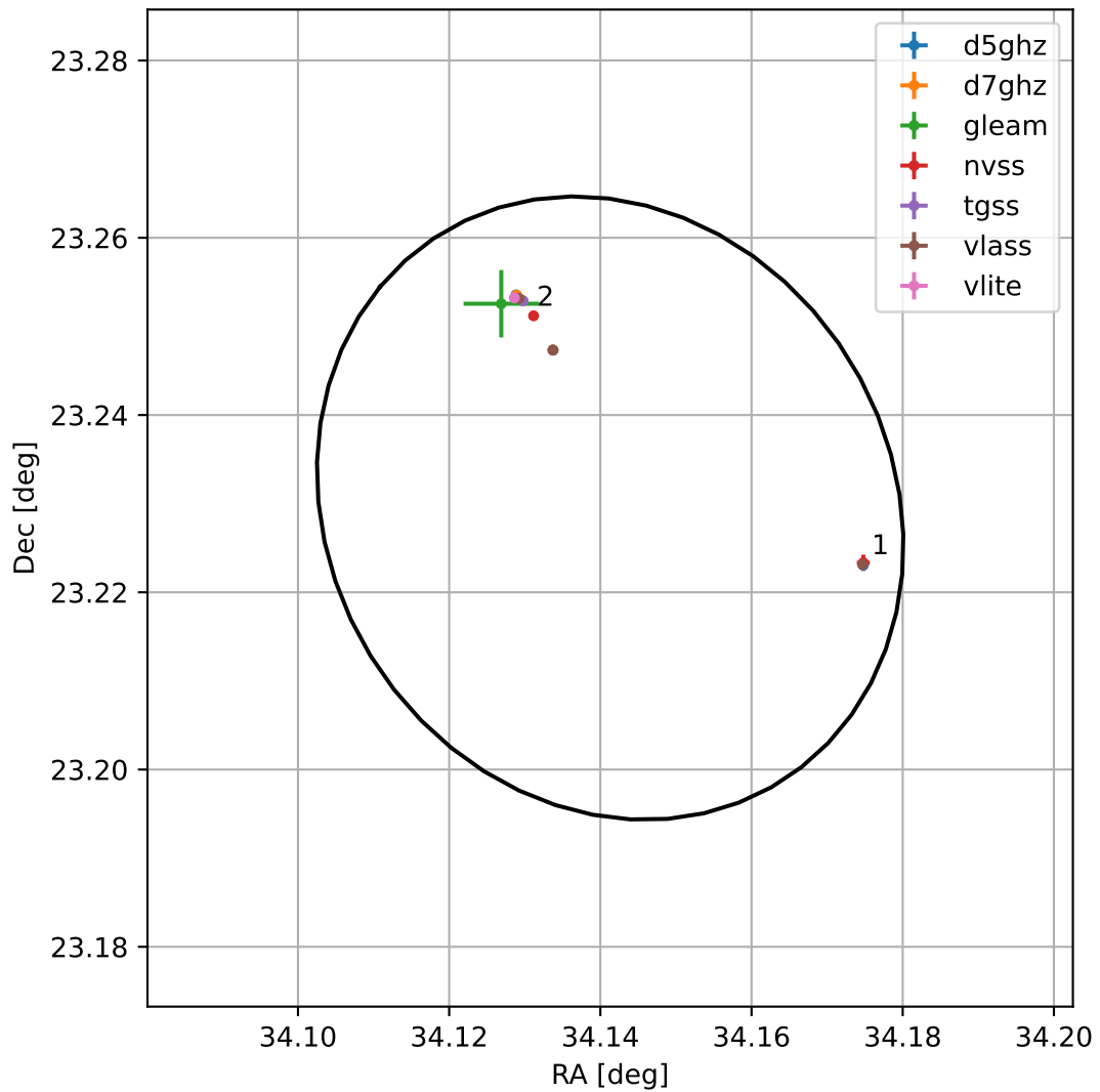
4FGL J0216.5+2313
