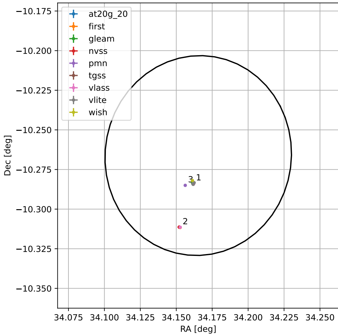
4FGL J0216.6-1015
