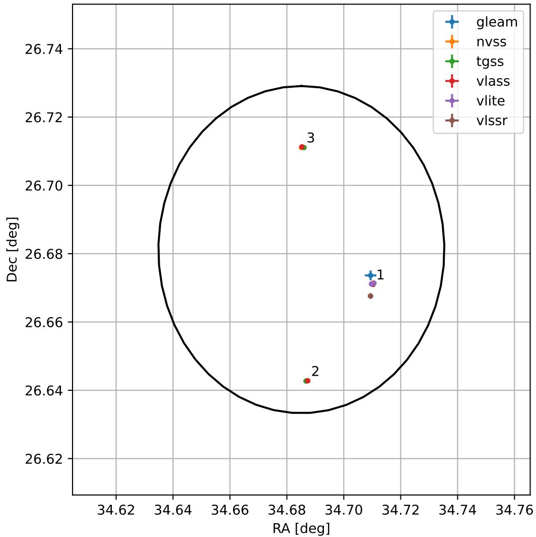
4FGL J0218.7+2640
