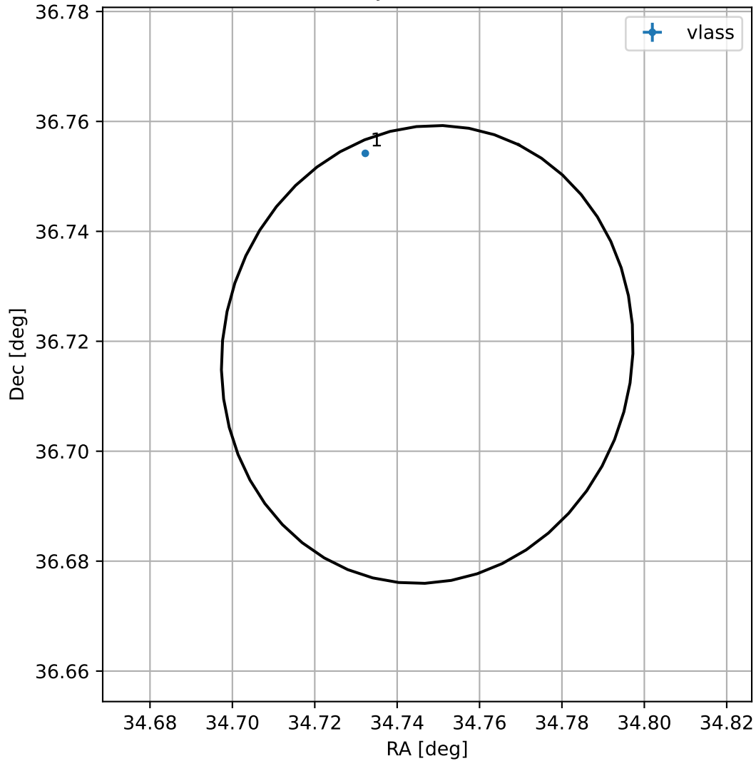
4FGL J0218.9+3643
