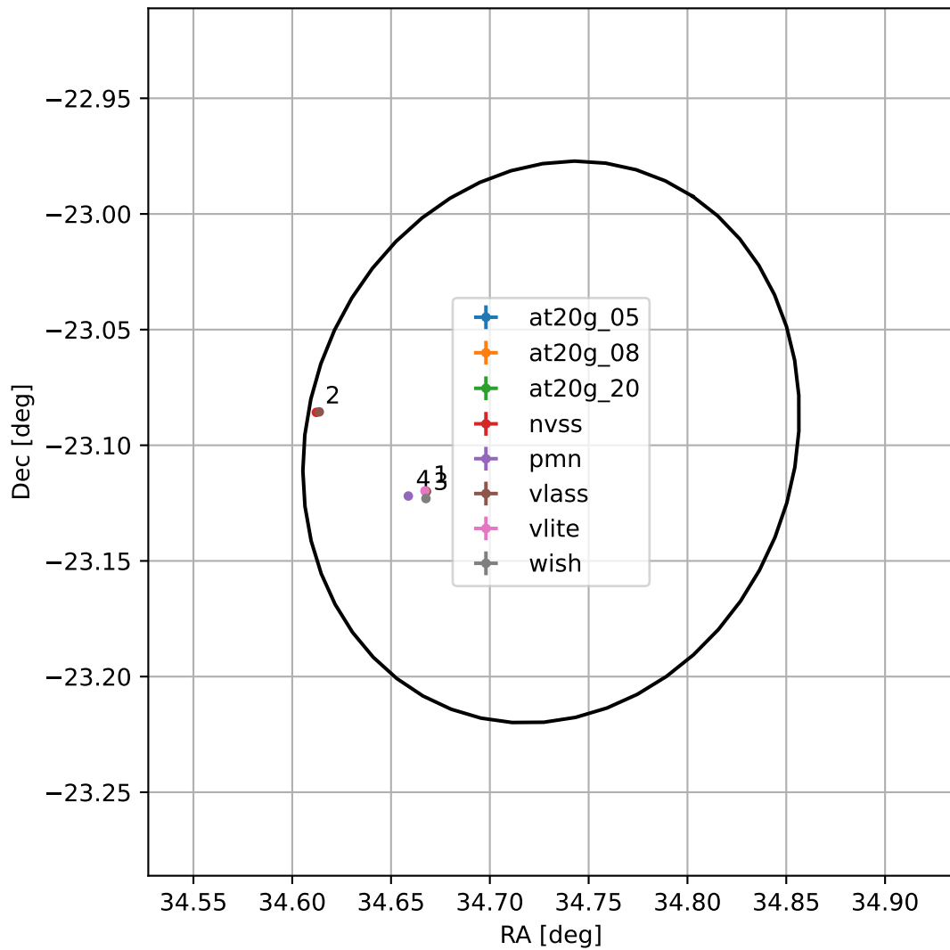
4FGL J0218.9-2305
