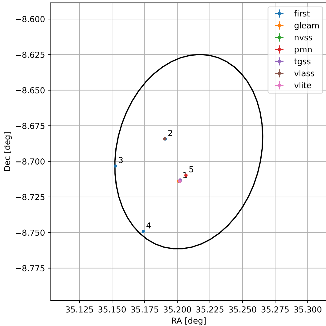
4FGL J0220.8-0841
