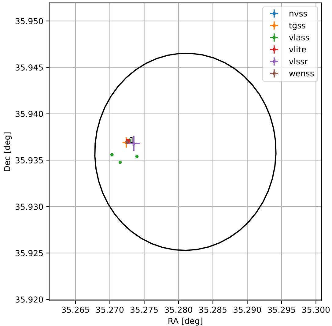
4FGL J0221.1+3556
