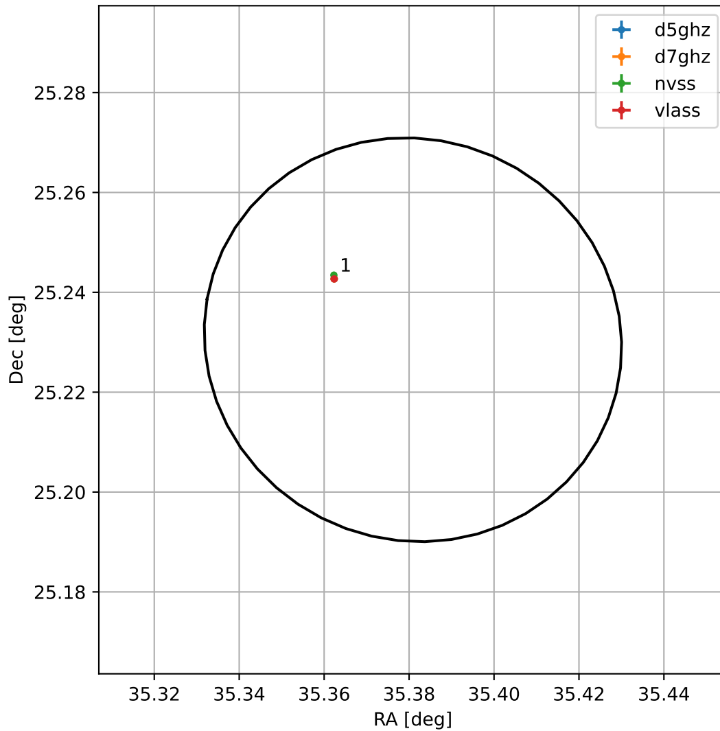
4FGL J0221.5+2513
