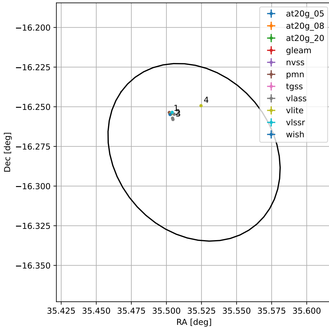
4FGL J0222.0-1616
