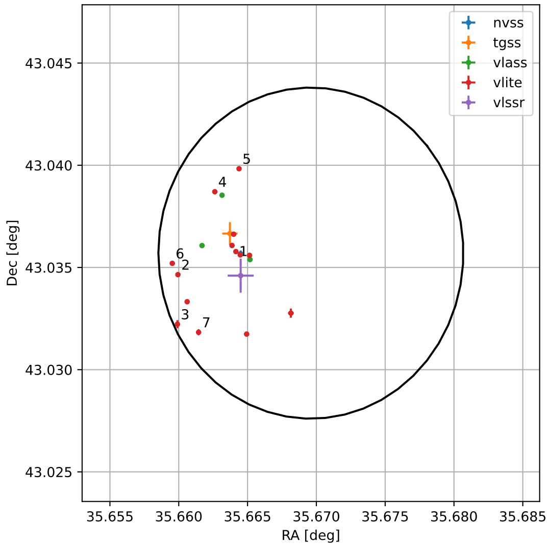
4FGL J0222.6+4302
