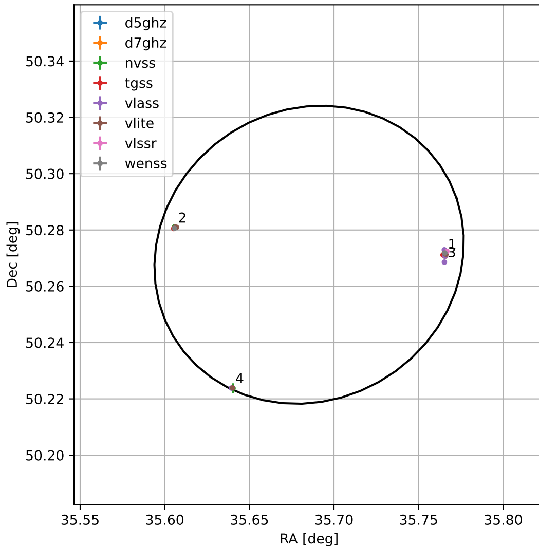
4FGL J0222.7+5016
