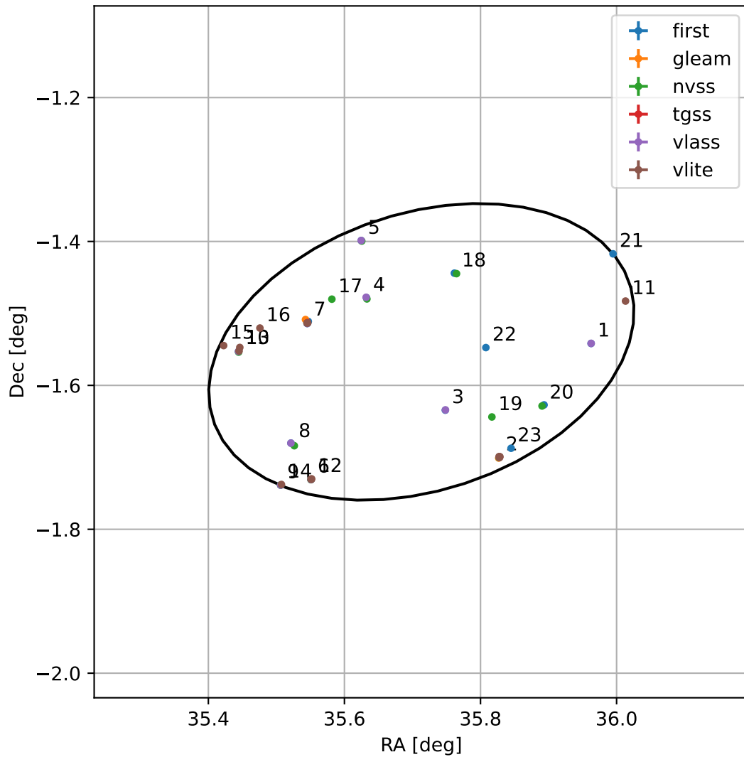
4FGL J0222.8-0133
