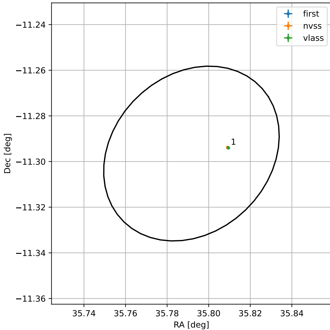
4FGL J0223.1-1117
