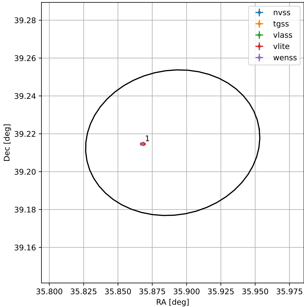
4FGL J0223.5+3912
