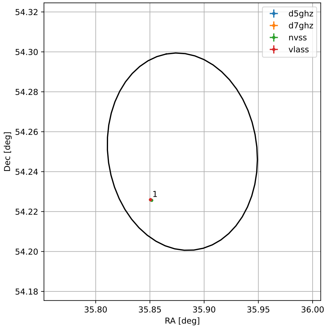
4FGL J0223.5+5415
