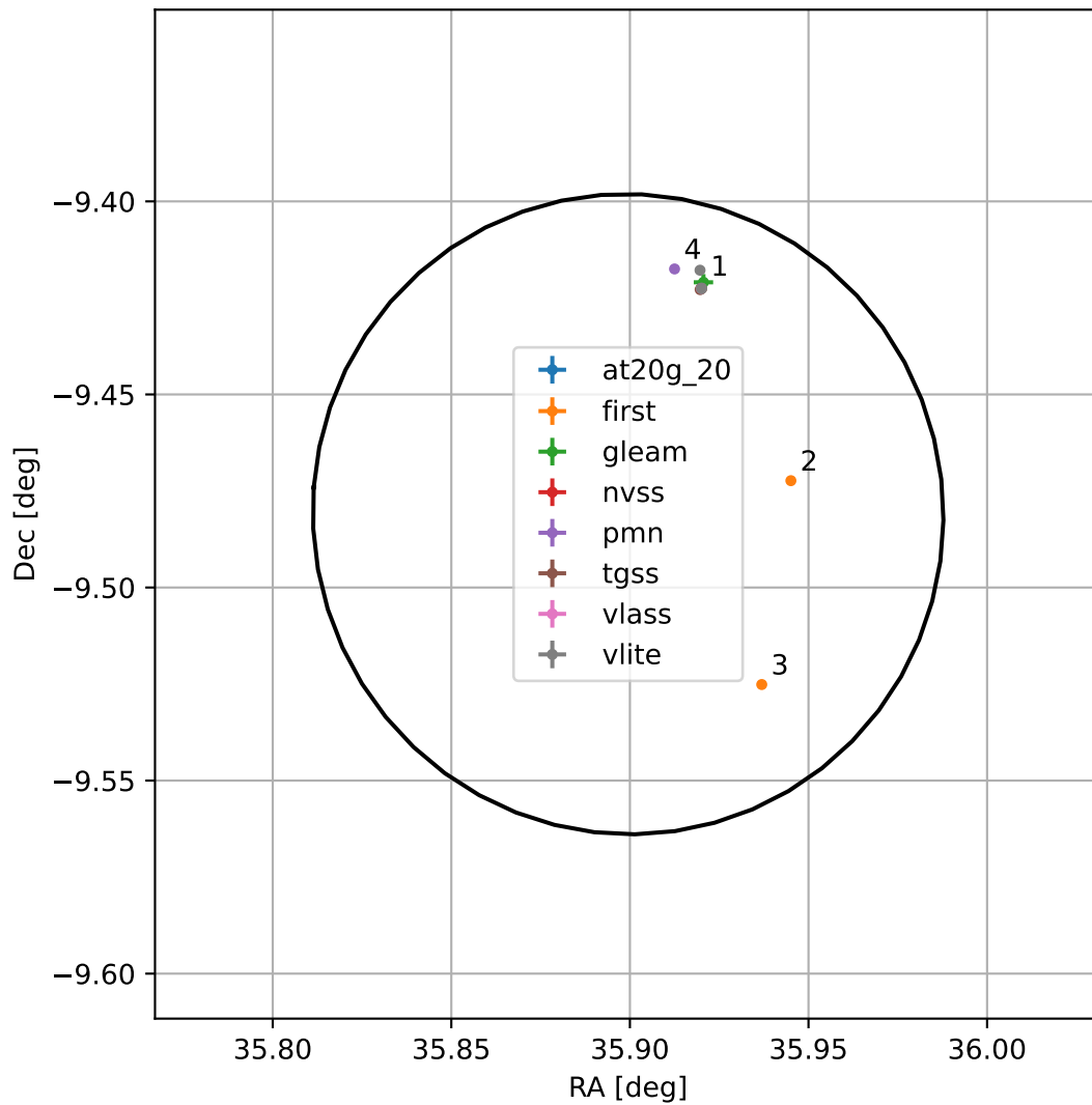
4FGL J0223.5-0928
