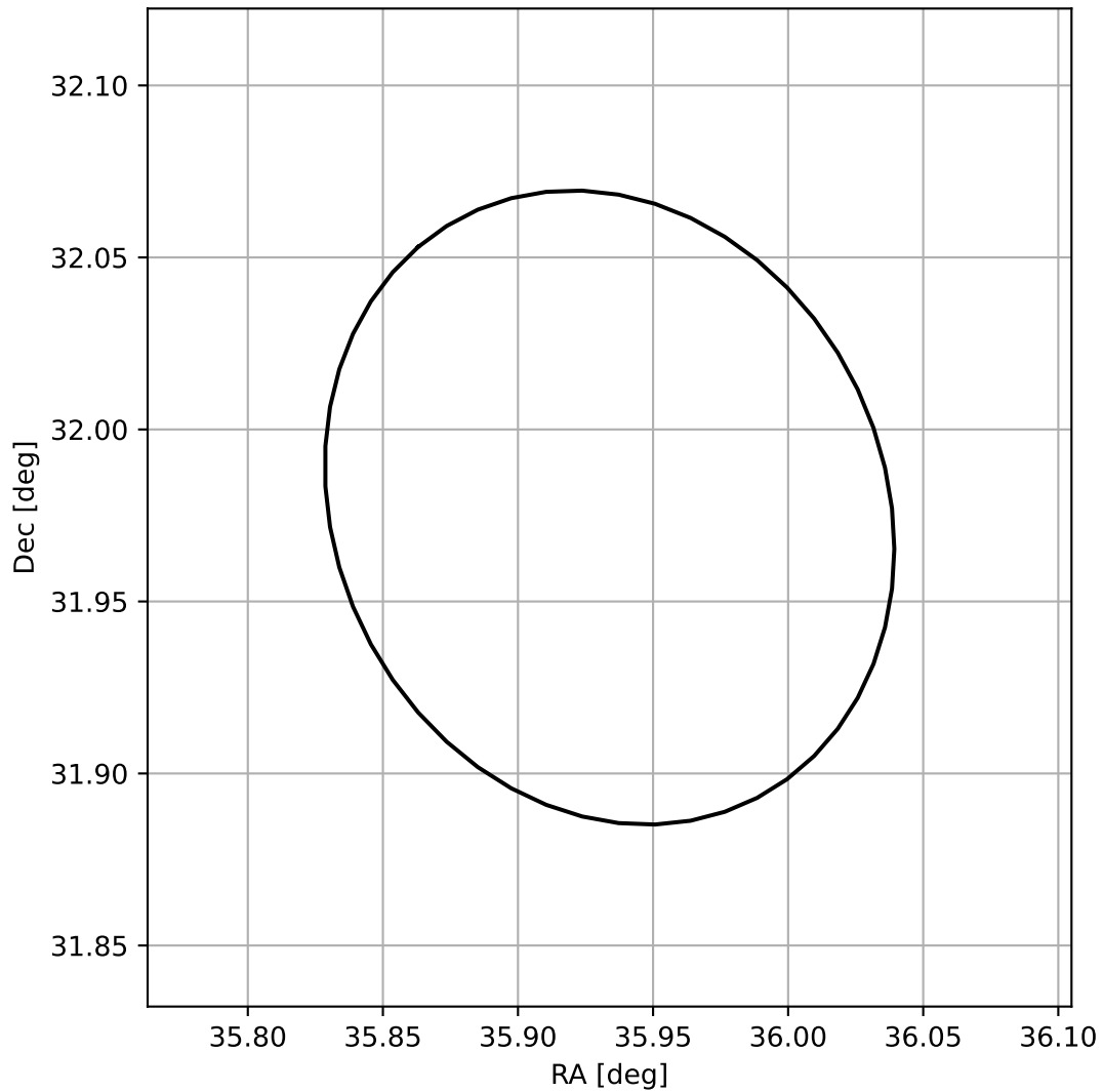
4FGL J0223.7+3158
