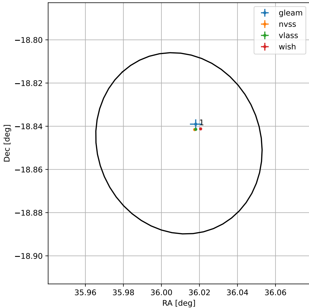
4FGL J0224.0-1850
