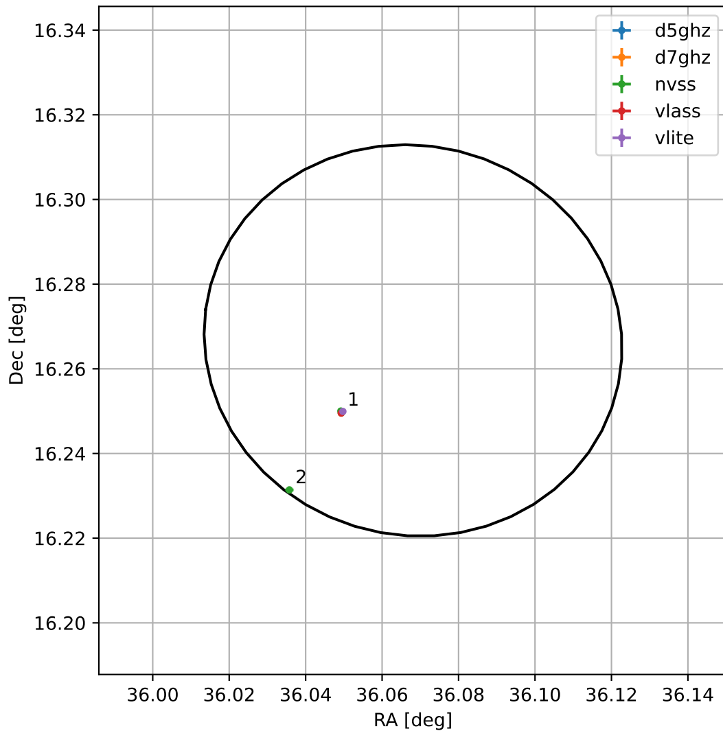
4FGL J0224.2+1616
