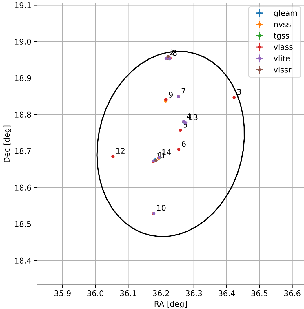
4FGL J0224.9+1843
