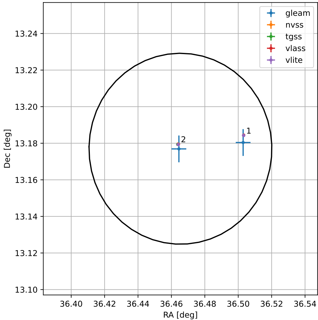
4FGL J0225.8+1310
