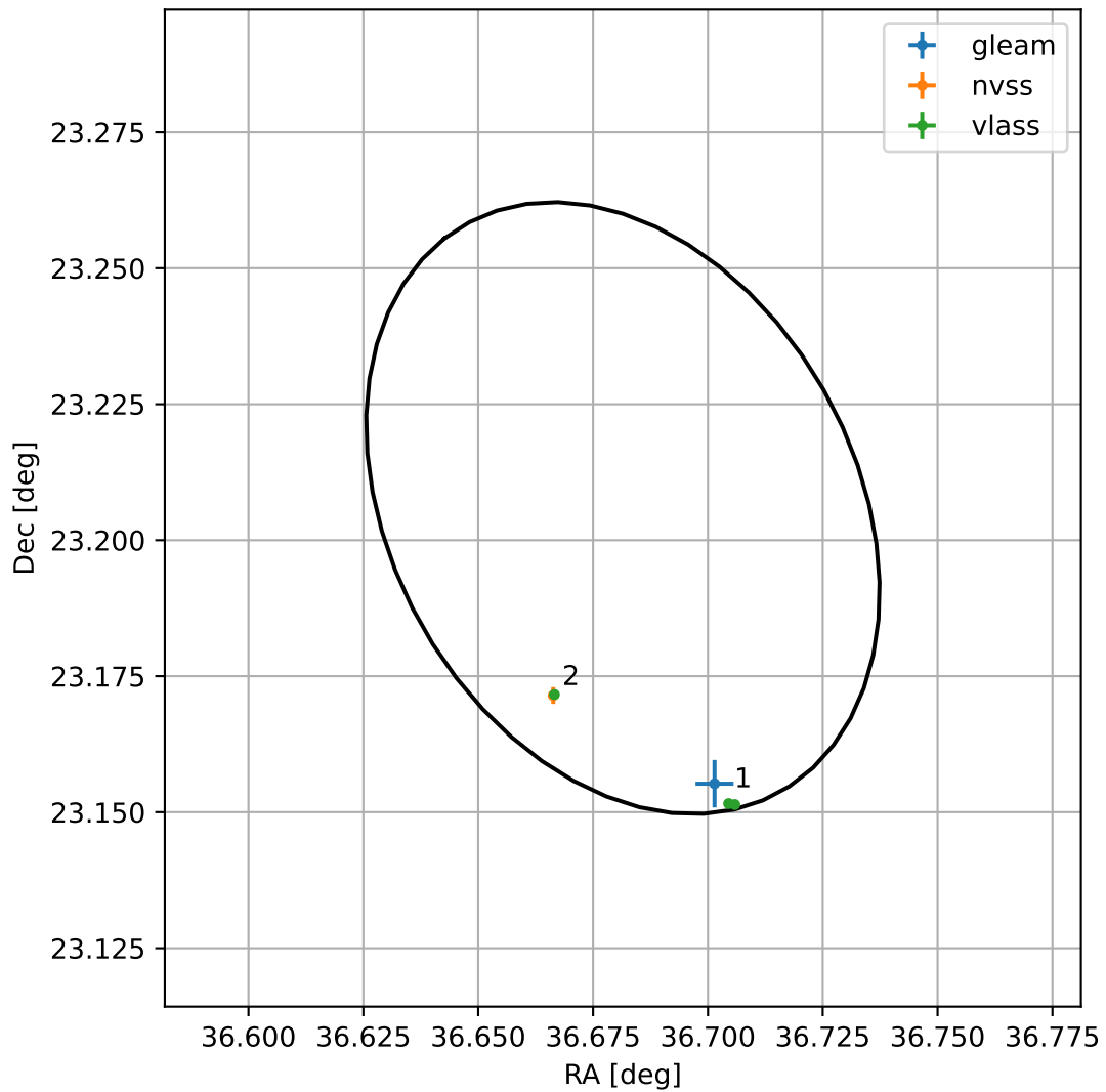
4FGL J0226.7+2312
