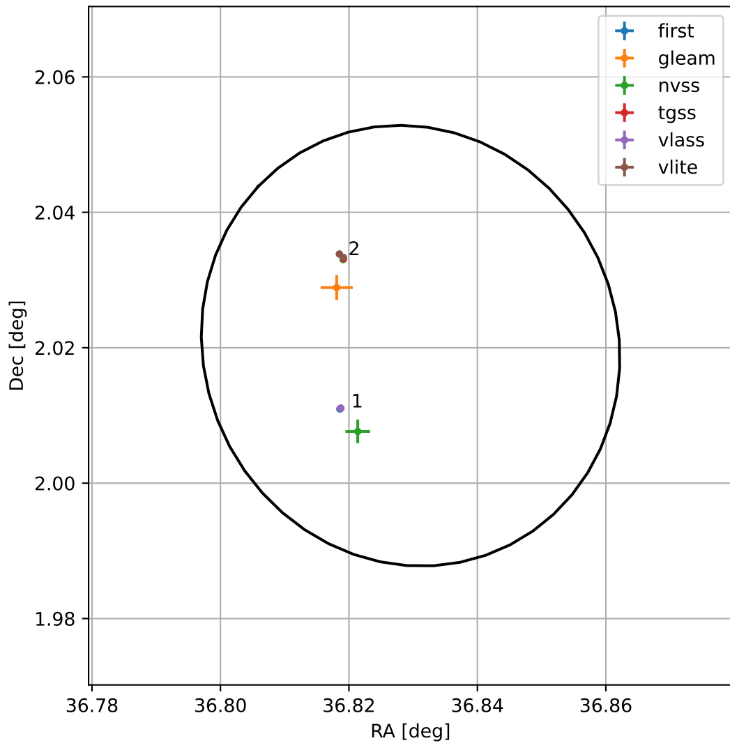
4FGL J0227.3+0201
