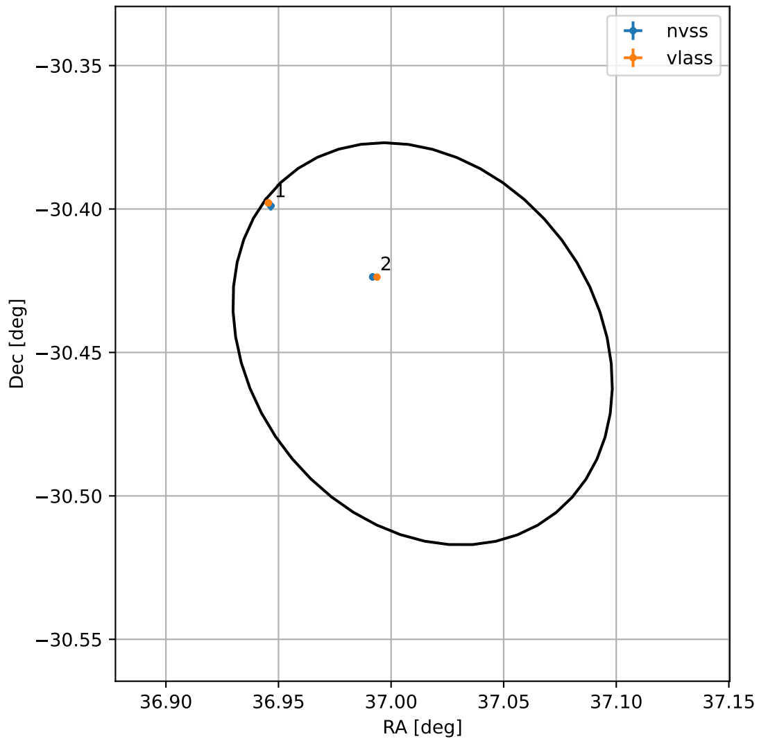
4FGL J0228.0-3026
