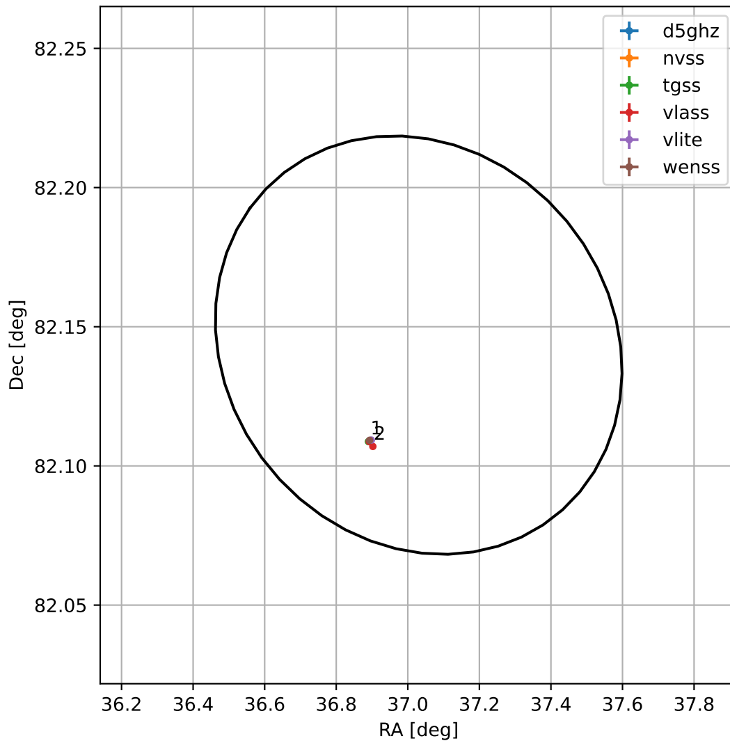
4FGL J0228.1+8208
