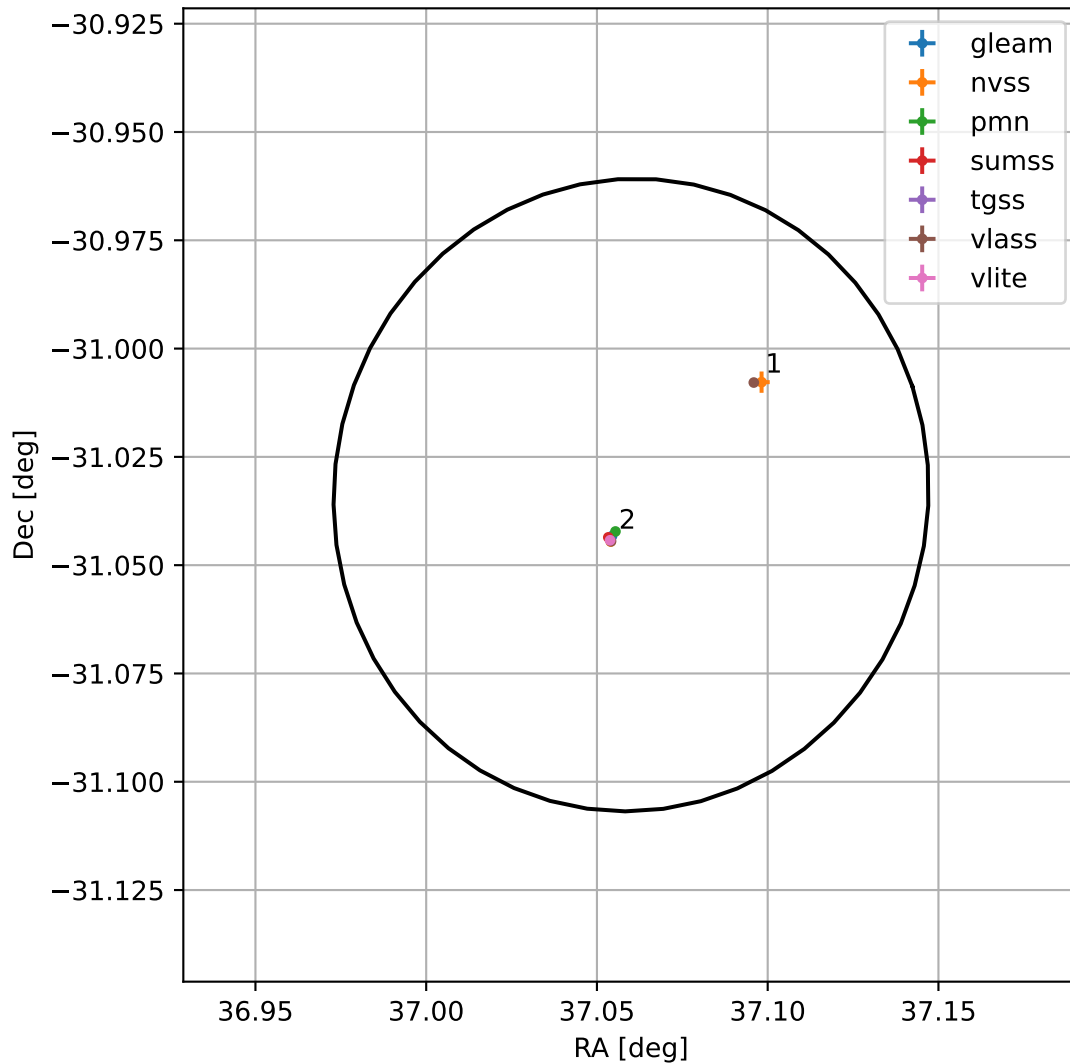
4FGL J0228.2-3102
