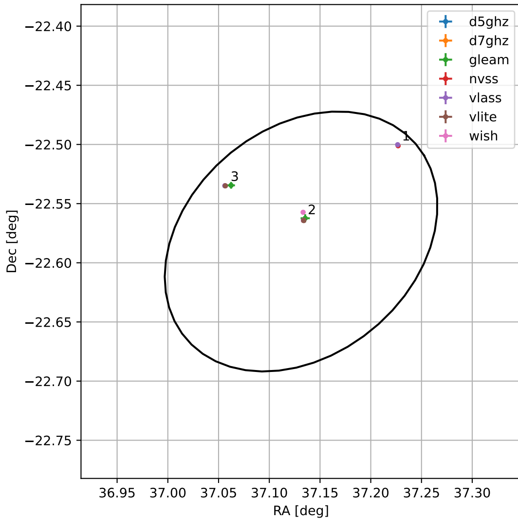
4FGL J0228.5-2234
