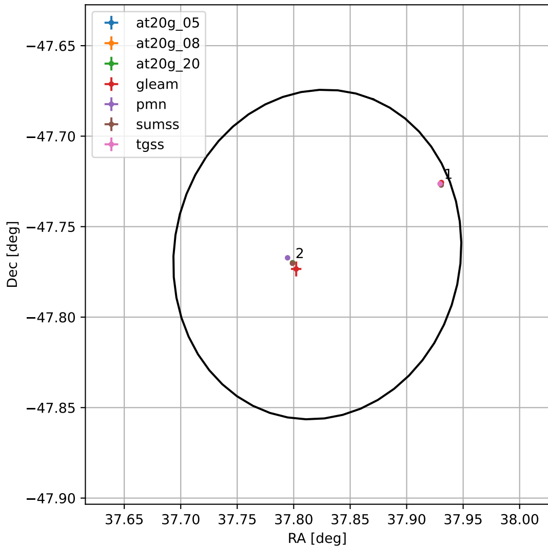
4FGL J0231.2-4745
