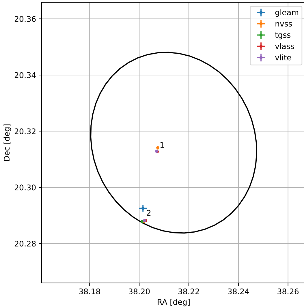
4FGL J0232.8+2018
