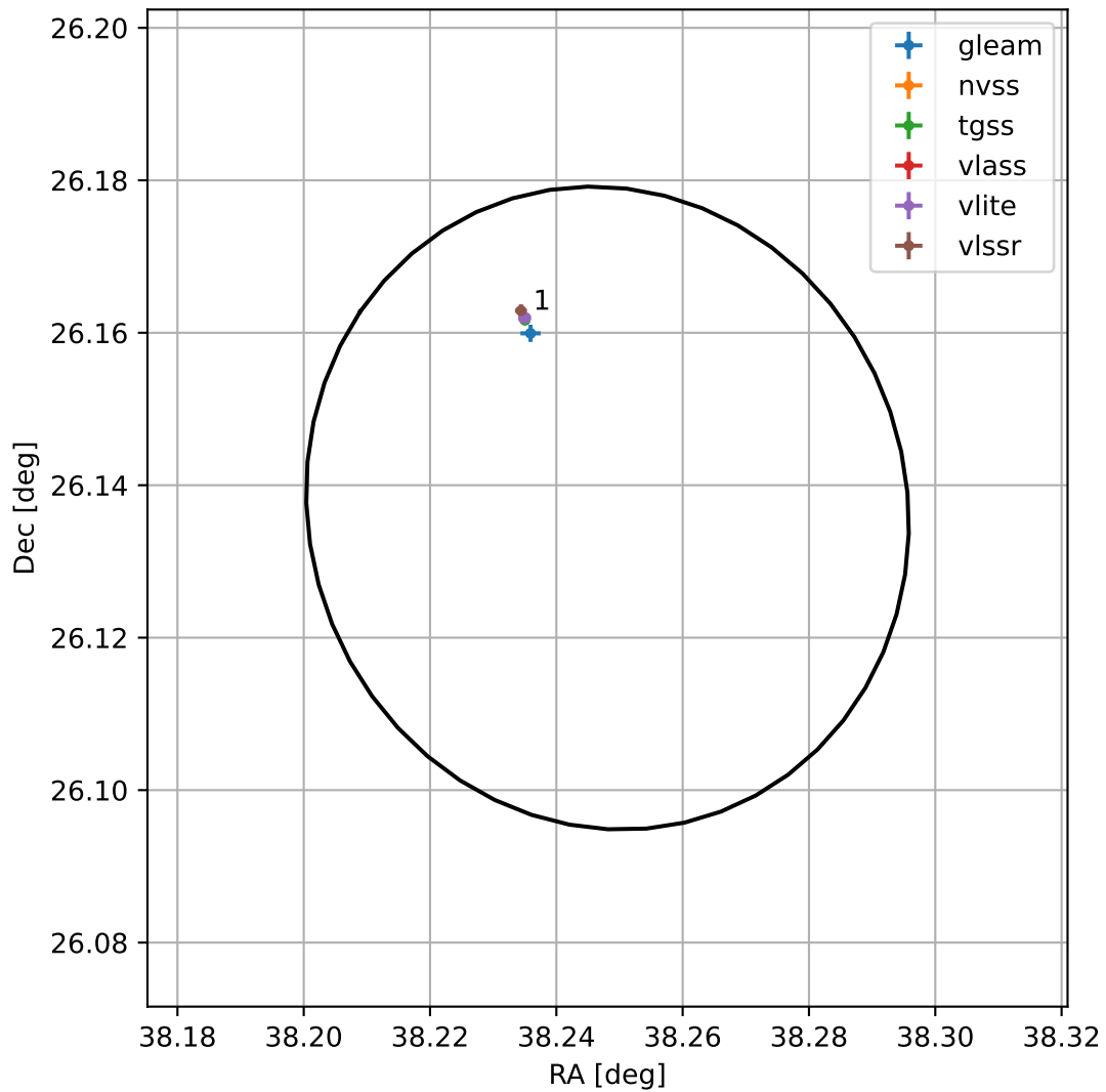
4FGL J0232.9+2608
