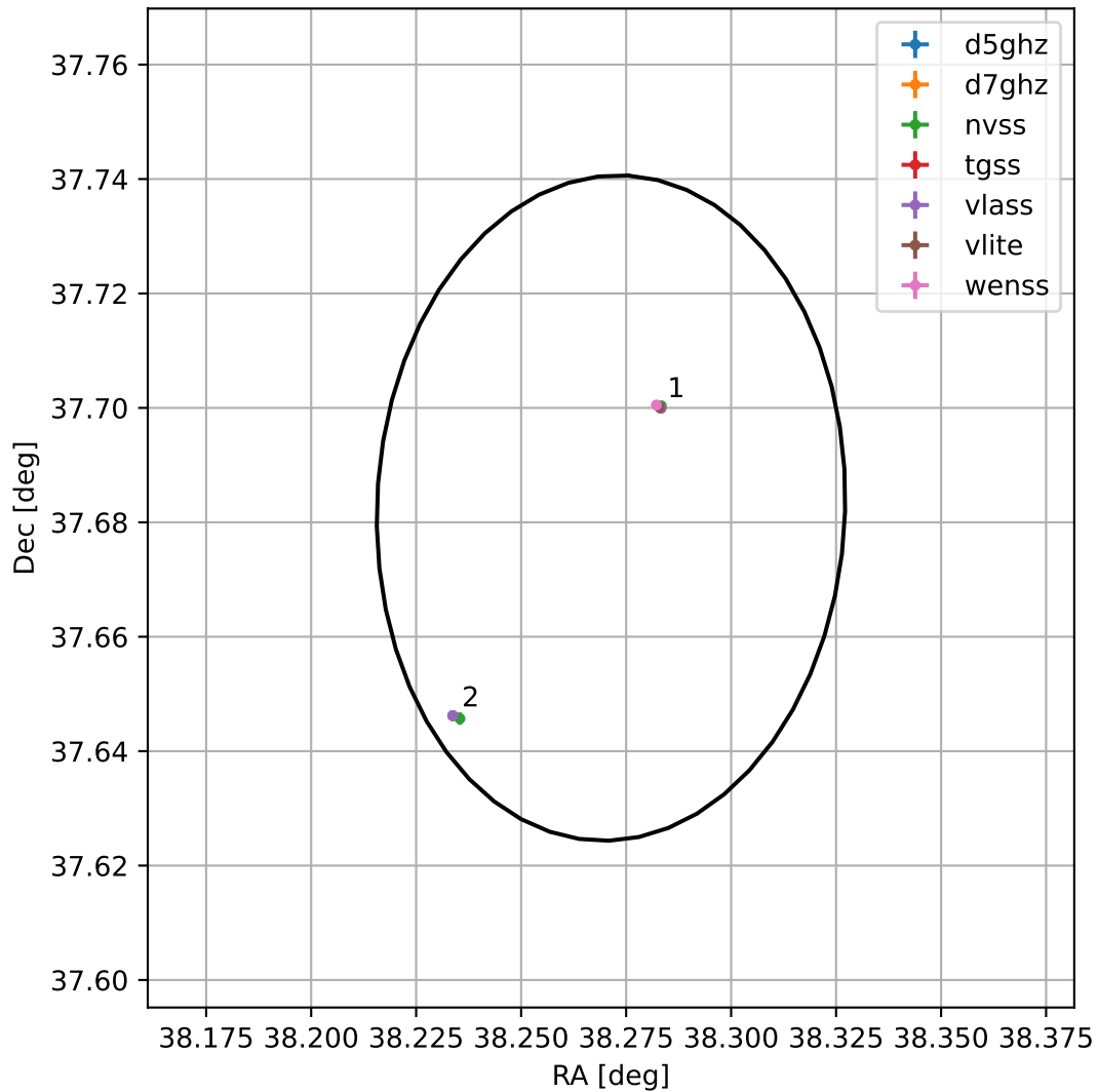
4FGL J0233.0+3740
