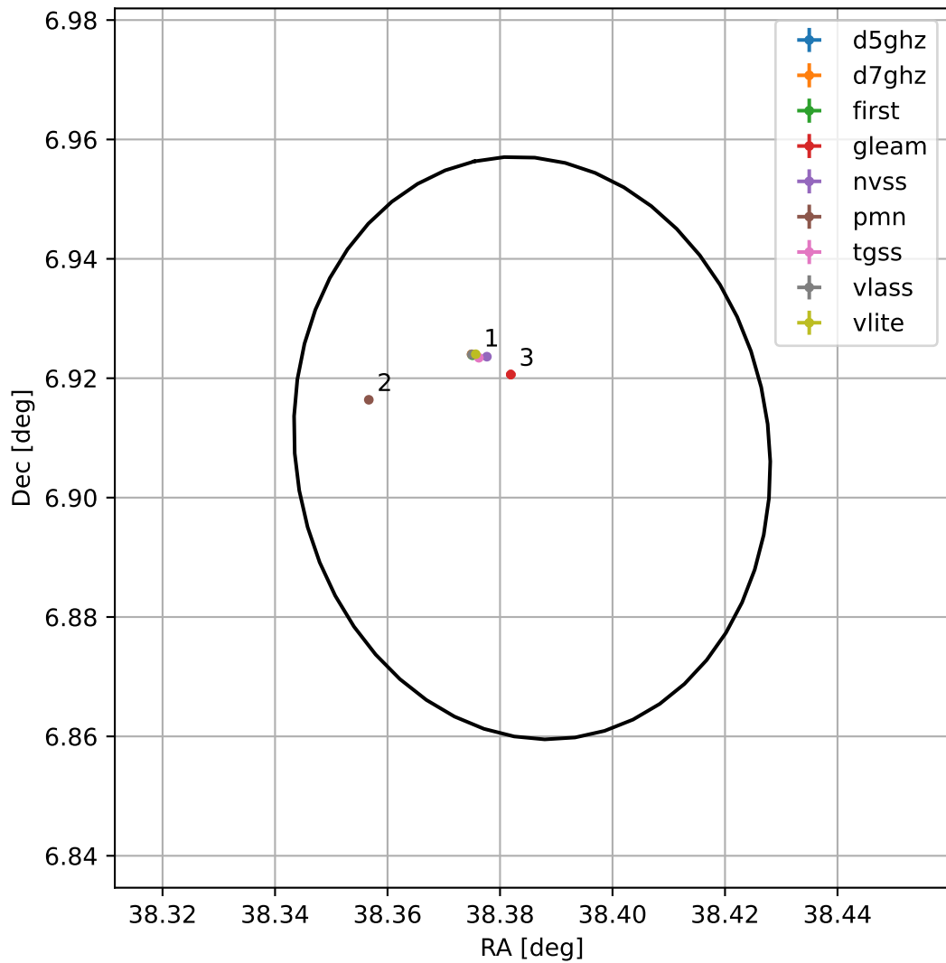
4FGL J0233.5+0654
