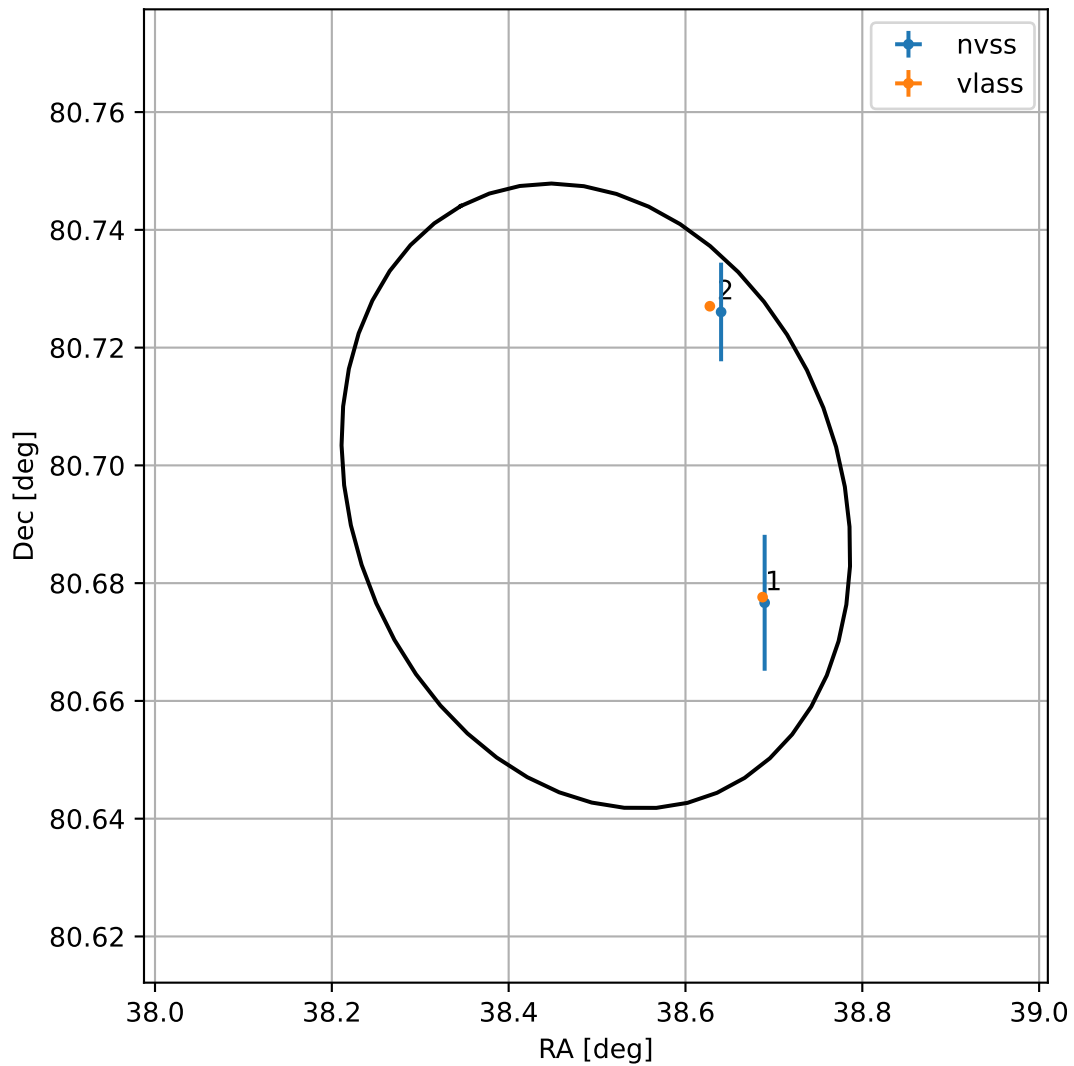
4FGL J0233.9+8041
